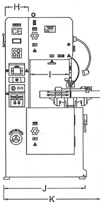
SVR400 Dimensions of Various Parts scale: mm
