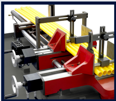
MECHANICAL BUNDLE CLAMPING DEVICE (OPTIONAL)
