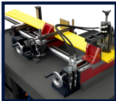
HYDRAULIC BUNDLE CLAMPING (OPTIONAL)
