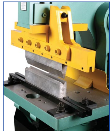
OPTIONAL PRESSBRAKE TOOL HOLDERS
